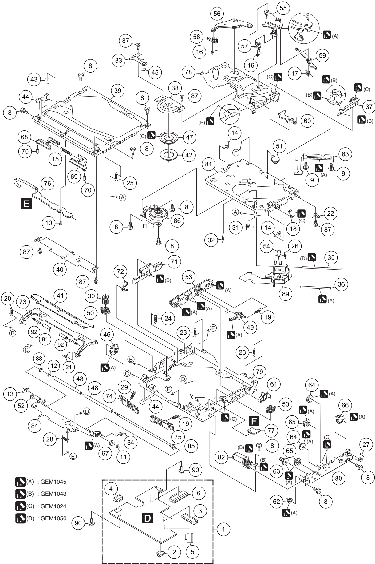
AVH-P5000DVD/XN/UC
